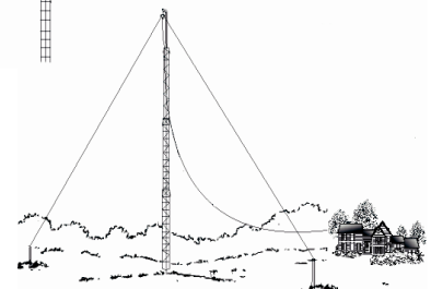
ABOVE: INVERTED "V" CONFIGURATION
